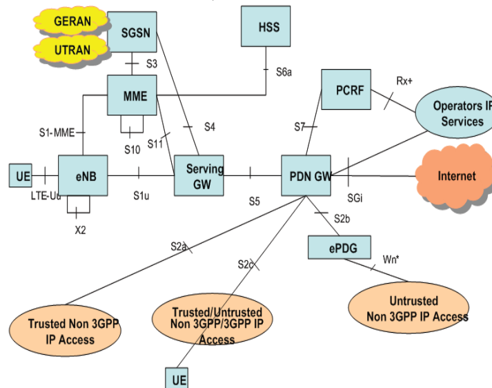
Fig. 1 LTE Architecture Overview UE
