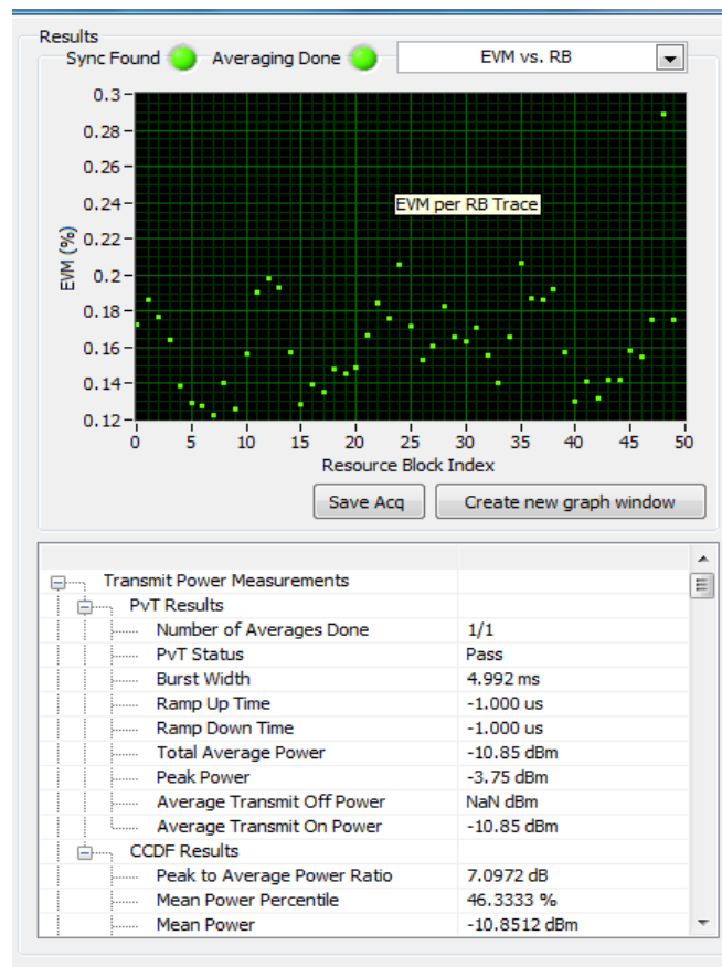
Fig. 4 Error Vector Magnitude
