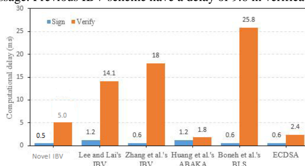
Fig.2 Comparison of computational delay to verify and signing message
