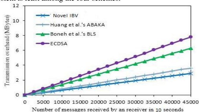
Fig.3 Transmission overhead with number of message received
