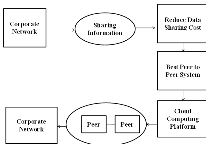
Figure 1: Architecture Diagram
