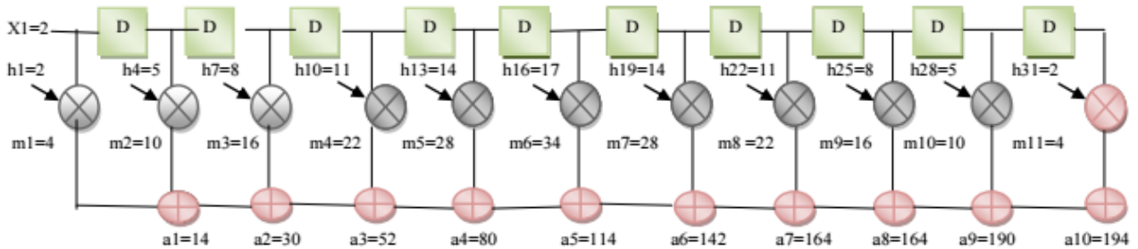
Figure 3: Internal Structure of H1
