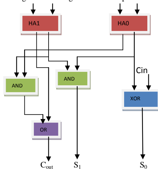
Figure 3: Logic diagram of modified 2 bit KS adder
