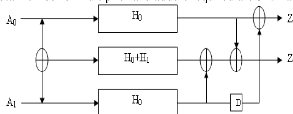
Figure 1: Parallel 2x2 FIR Filter
