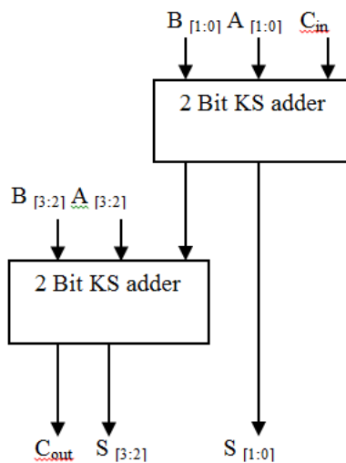
Figure 4: Proposed 4-bit KS adder
