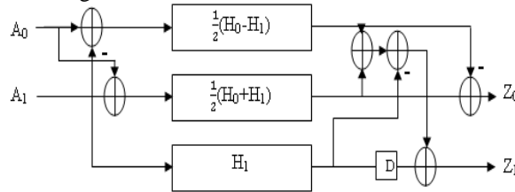
Figure 2: Proposed Parallel 2x2 FIR Filter
