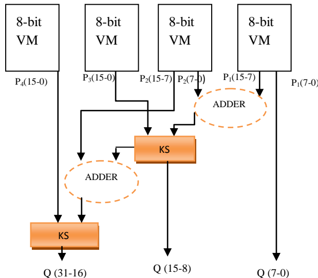
Figure 2: Proposed 16x16 Vedic Multiplier
