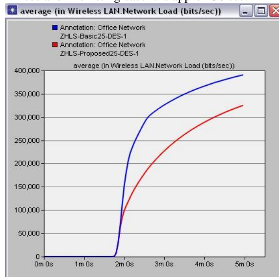
Figure 4.6 Network Load
