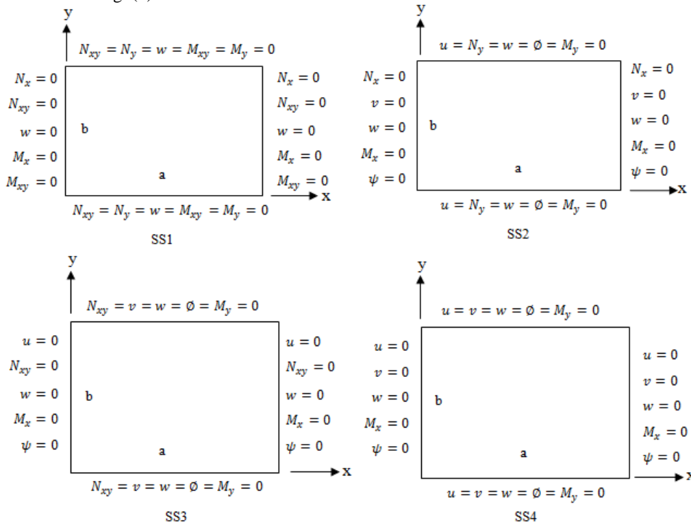
Fig. (1) Simply supported boundary conditions
