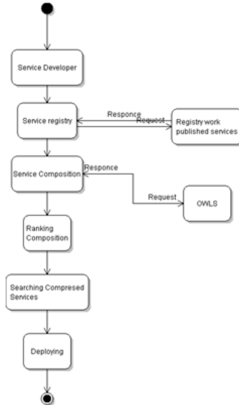
Fig 1: Shows the Scalable web service Composition
