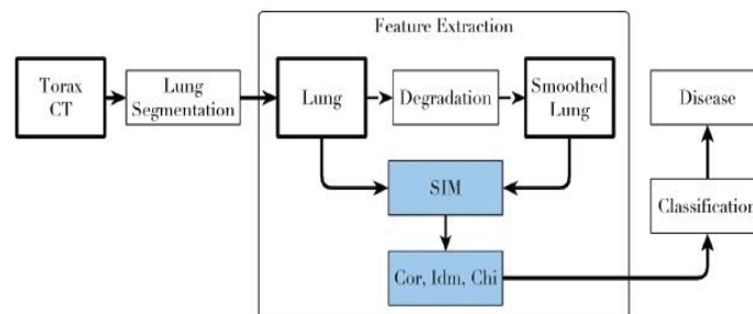
Figure 1. Model for the proposed pulmonary disease classification.
