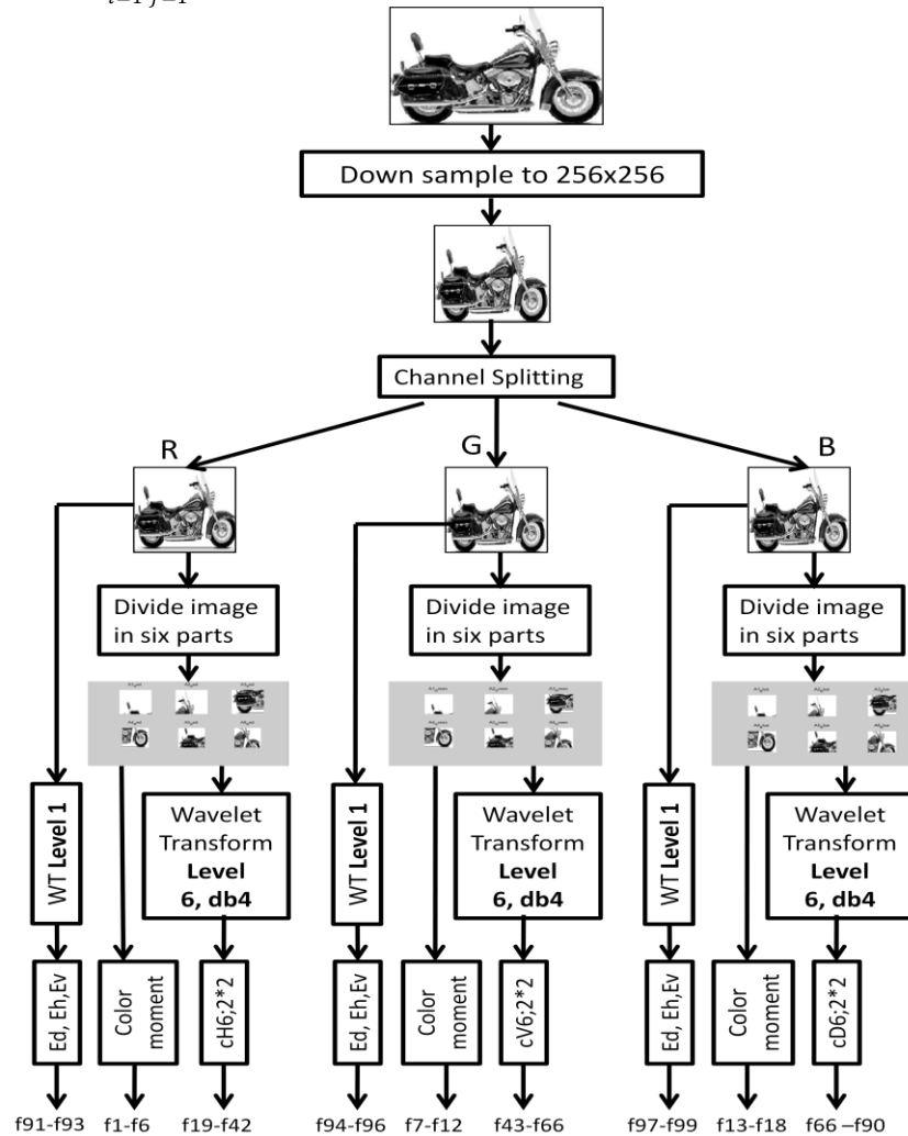
Fig. 4 Image feature extraction methodology
