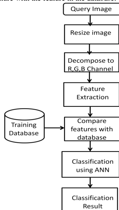
Fig. 3 Online process for Image classification using ANN
