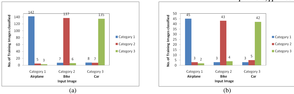
Fig. 5 Performance of ANN classifier for Images (a) Training images (b) Testing images
