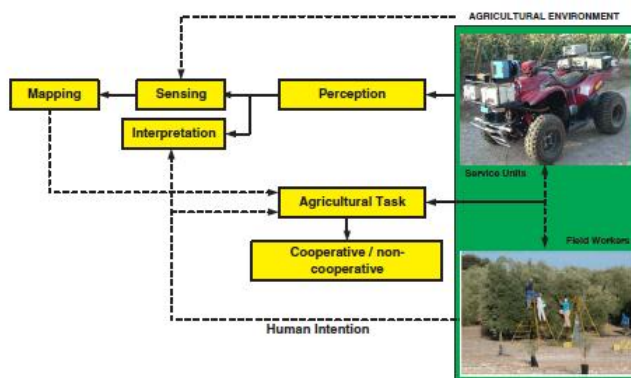
Fig 1. General architecture of an HRI for flexible robotic automation of farms.
