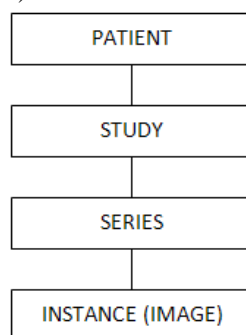
Fig. 14: DICOM Data Model
