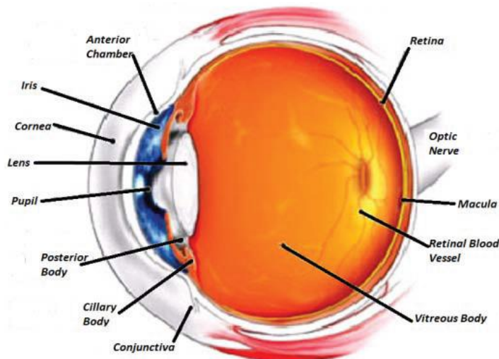
Fig.1 The eye anatomy
