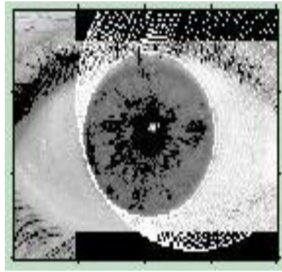
Fig.7 Normalized Image
