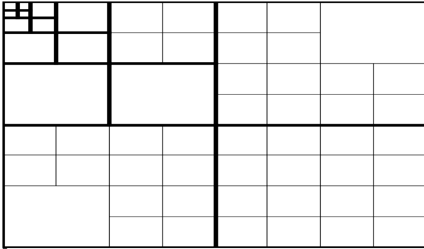
Wavelet packet structure drawn by 'S' subband
