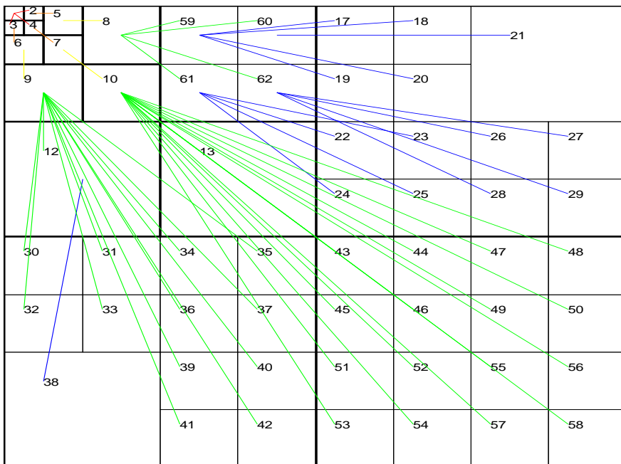
Wavelet packet structure drawn by 'S' subband
