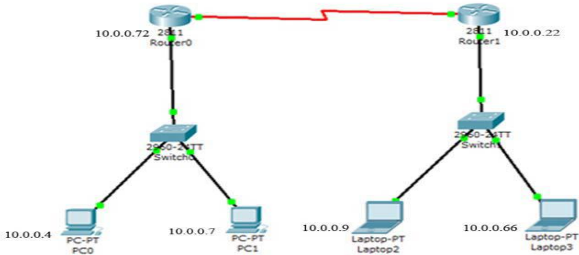
Fig 2.3 RIP configuration with same class of IP
