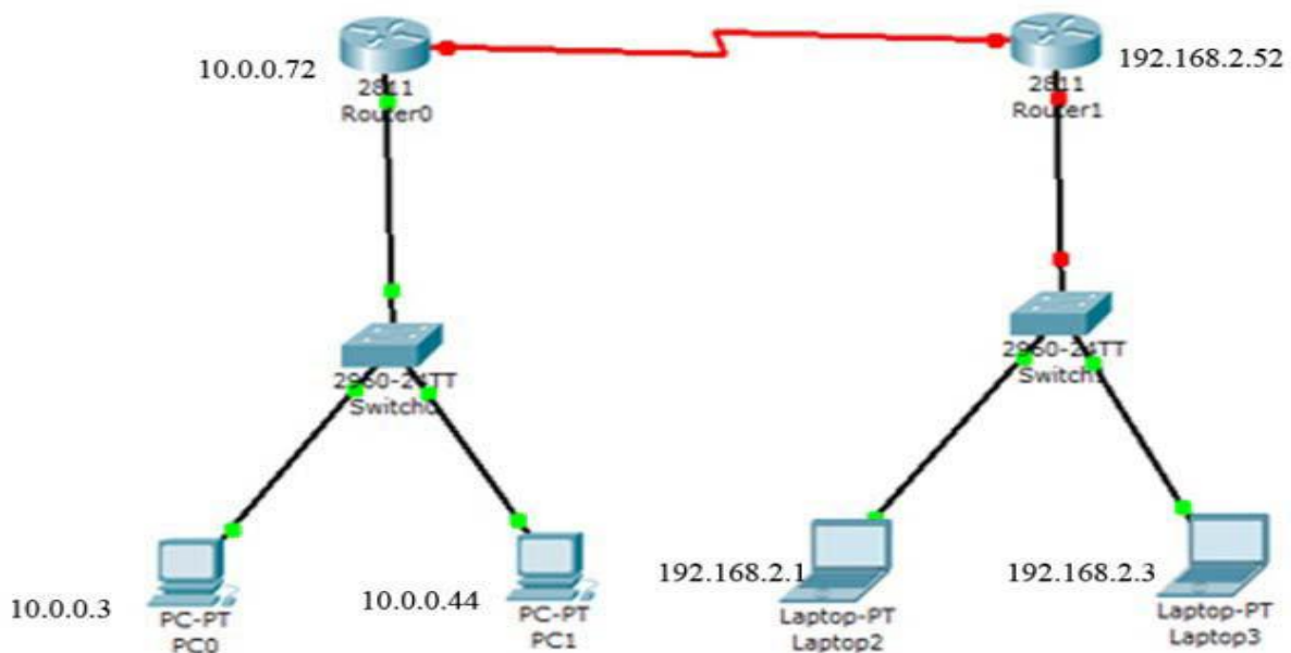
Fig 3.4 RIP configuration with different classes of IP
