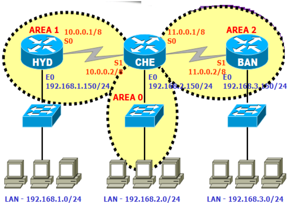
Fig 2.2 OSPF virtual Diagram
