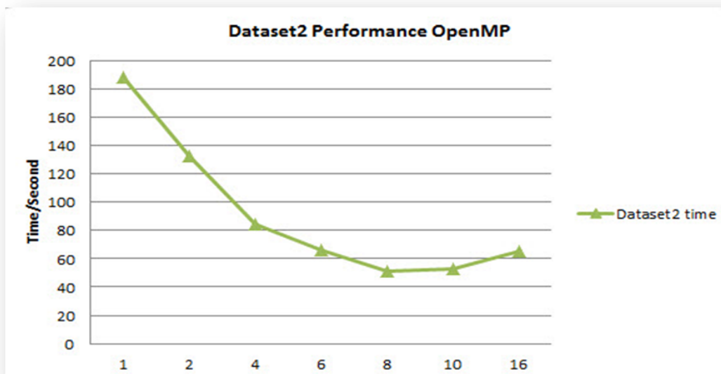
Fig. 4 shows the performance of OpenMP with Dataset 2
