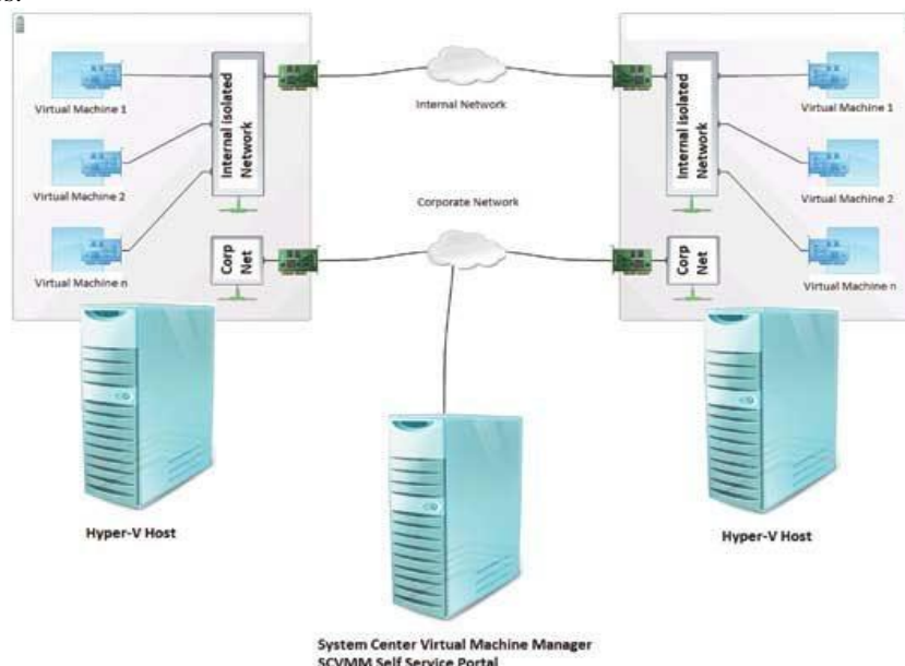
Figure 1: Cloud computing application with virtual machine process.
