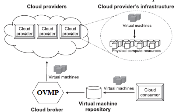
Figure 4: System model for optimized cloud environment.
