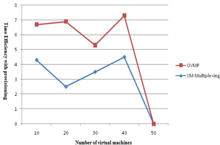
Figure 5: Comparison analysis of two different algorithmic analyses.
