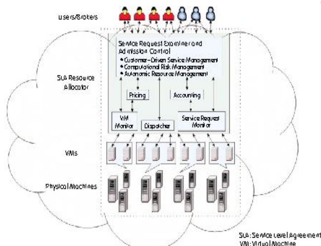
Figure 3: High level specification of the processing of resource provisioning in cloud computing.
