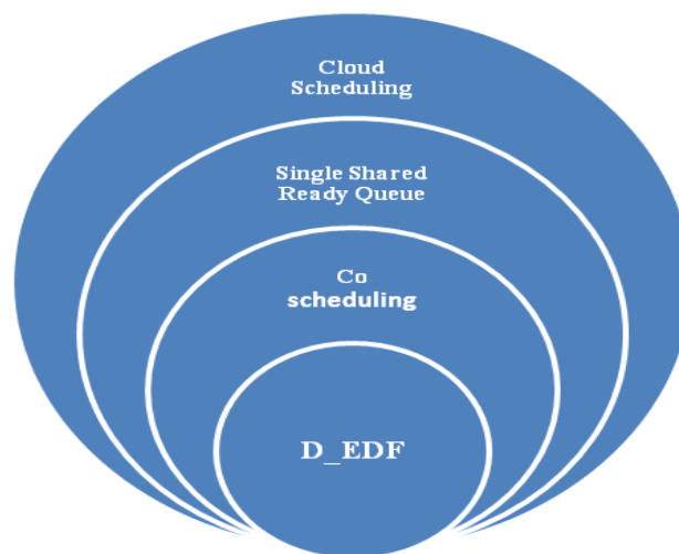
Fig. 3 scheduling schemes
