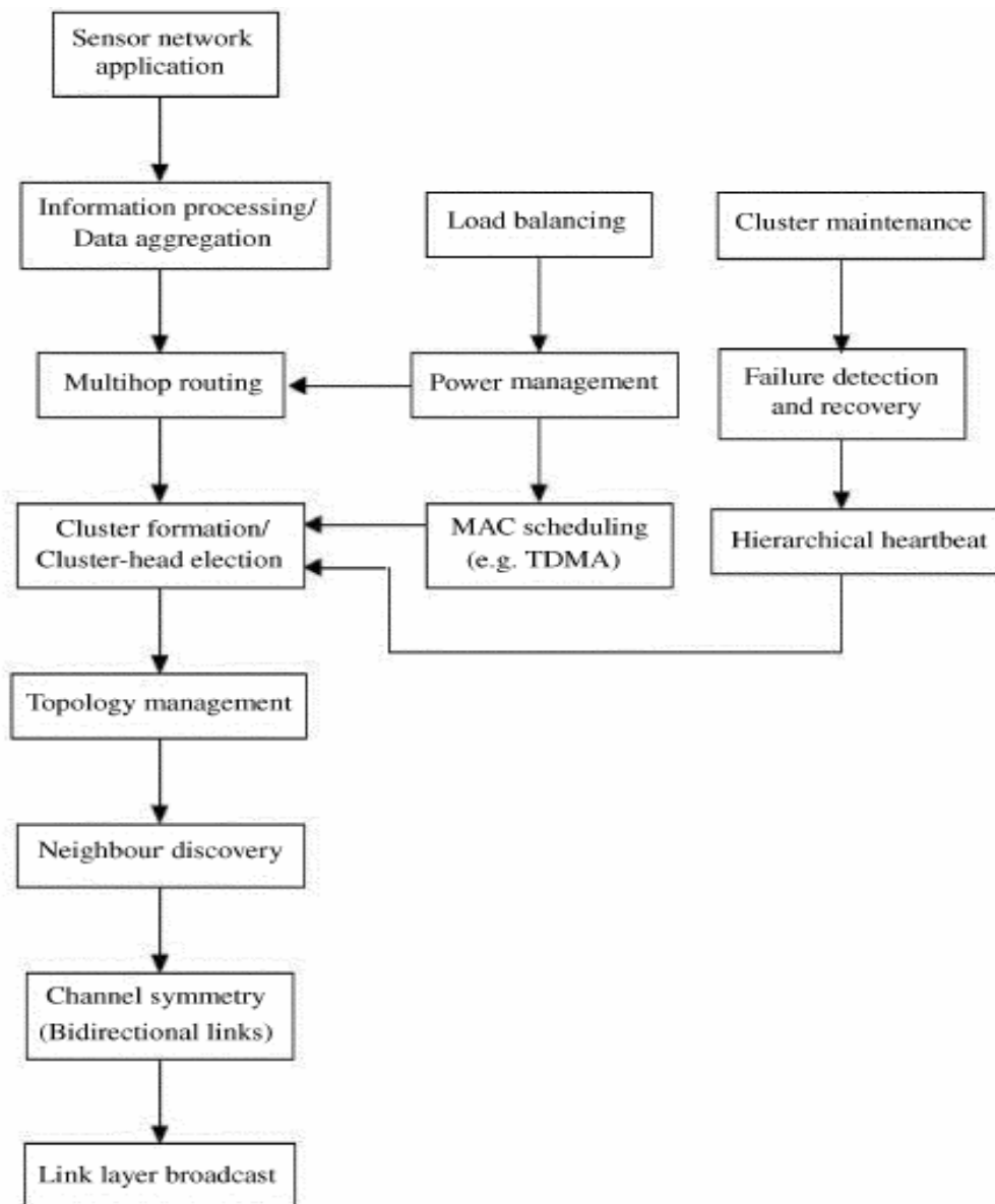
Fig.4 Depends-on hierarchy for cluster-based sensor network routing protocols. The function at the tail of an arrow depends on the function at the head of the arrow.
