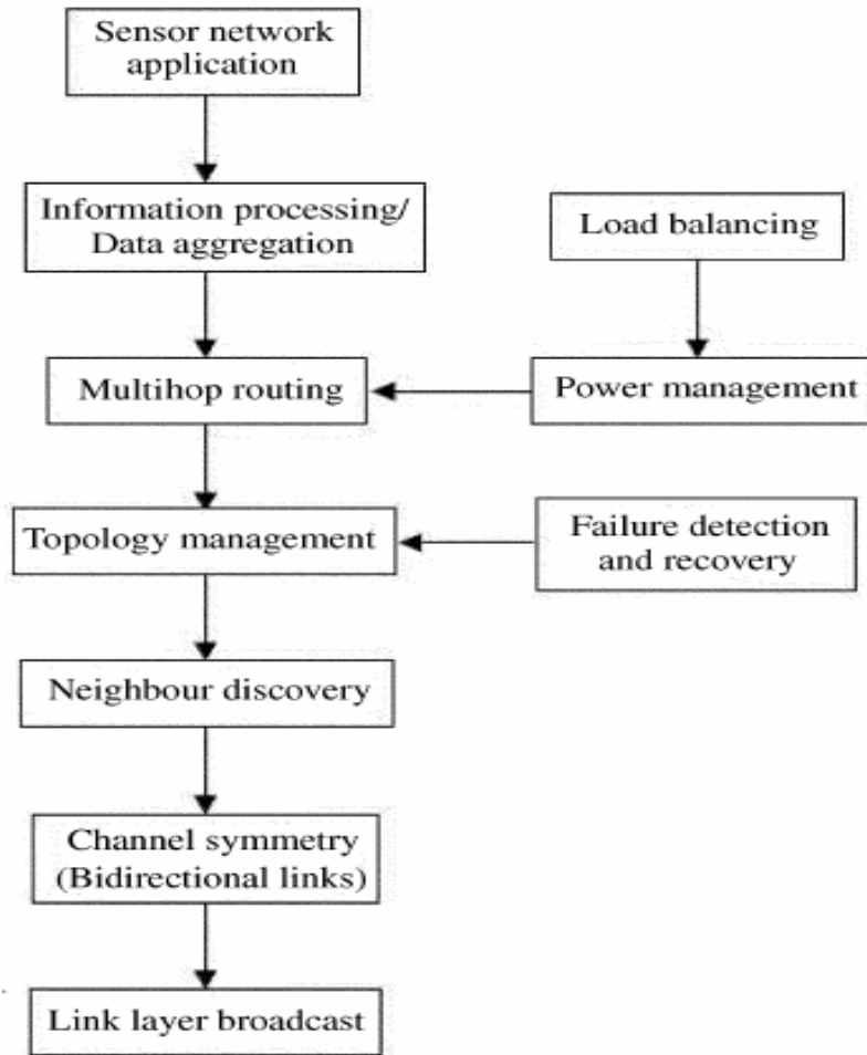
Fig.3. Depends-on hierarchy for flat sensor network routing protocols. The function at the tail of an arrow depends on the function at the head of the arrow.
