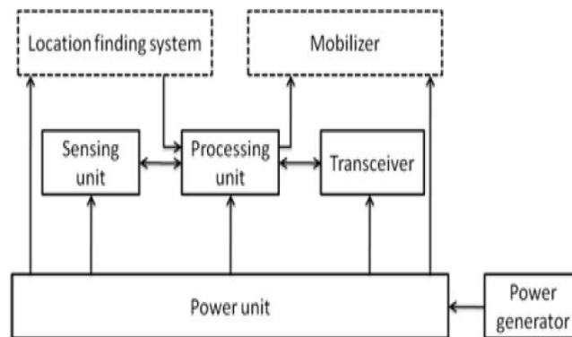
Fig. 1 Sensor node components
