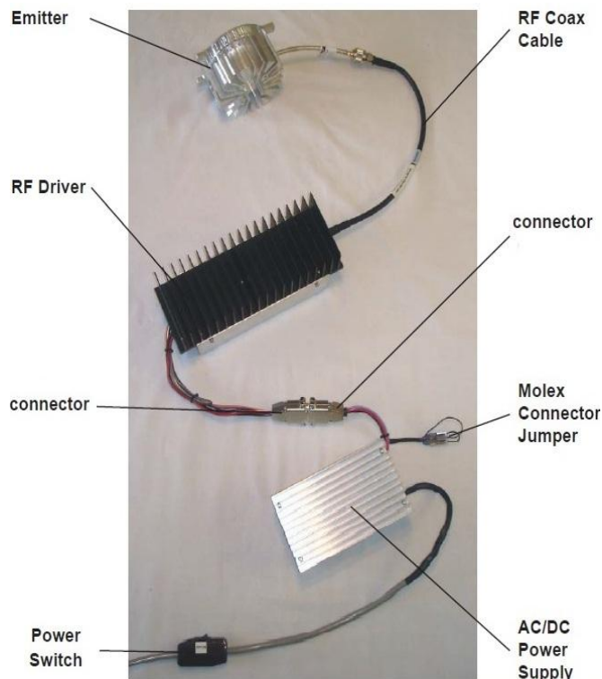
FIG.3.IMPLEMENTATION OF LI-FI
