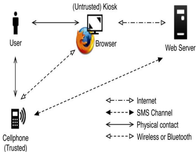
Fig. 1. Architecture of OPass system.
