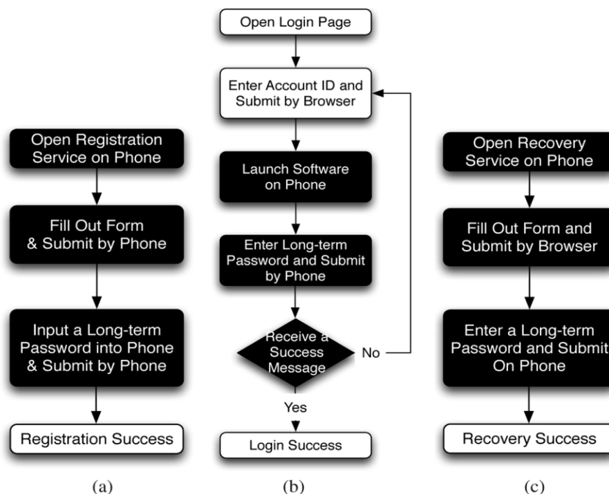
Fig. 2. Operation flows for user in every part of oPass system severally. Black rectangles indicate further steps contrasted with the generic authentication system: (a) registration, (b) login, and (c) recovery.
