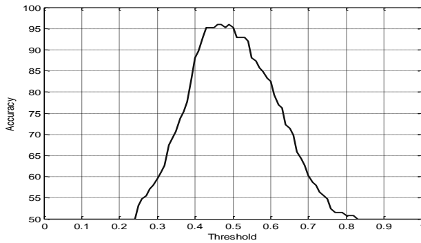
Figure 2 Accuracy graph for combined classifier
