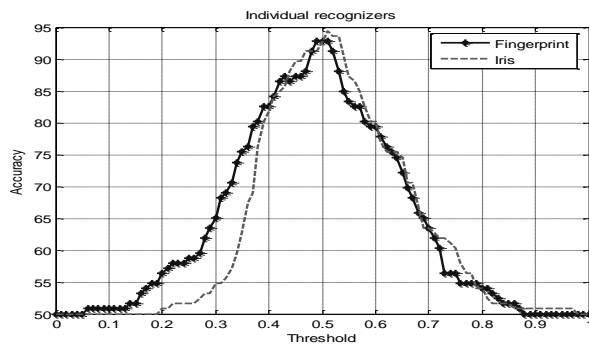
Figure 1 Accuracy plots of individual recognizers
