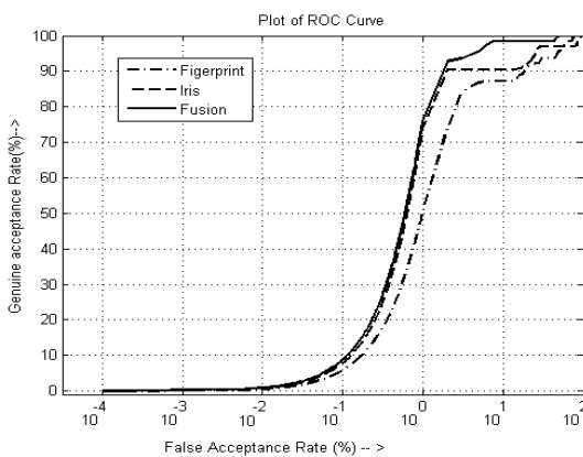
Figure 3 ROC Curve for Palmprint, Iris and Fusion
