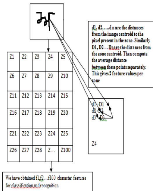
Figure 4 All procedure to extract feature from gurmukhi character image “Era (a)”.
