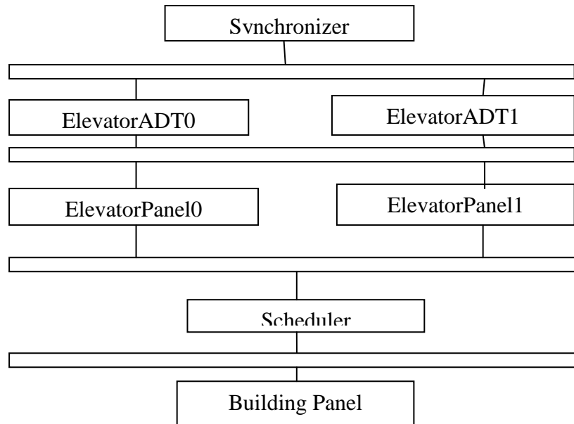
Figure 2. The Elevator C2 style architecture
