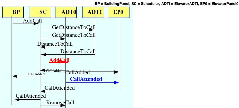
Figure 3: Architectural Test Case for the AddCall+CallAttended observation
