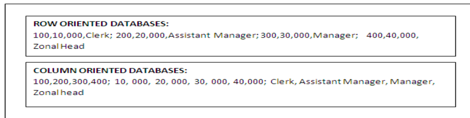
Figure 10: Representation of row and column oriented databases
