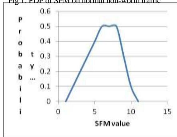
Fig 1: PDE of SFM on normal non-worm traffic
