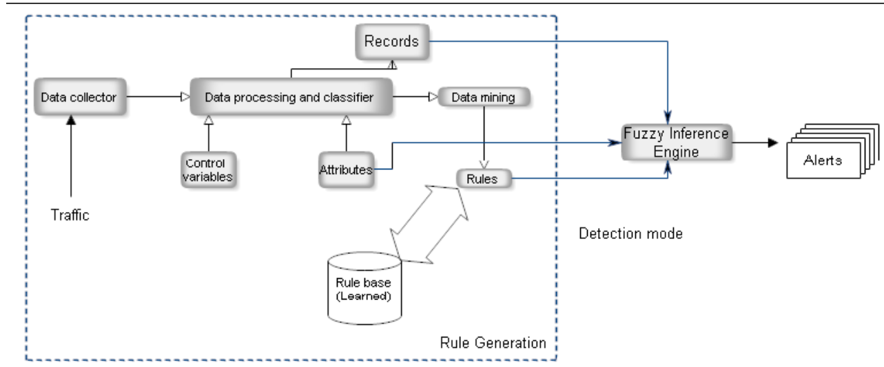
Figure 2. IIDS framework.
