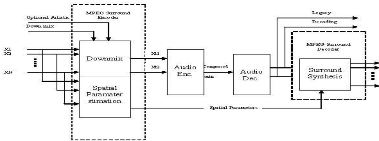
Fig . 9 Block diagram of encoding and decoding MPEG Surround
